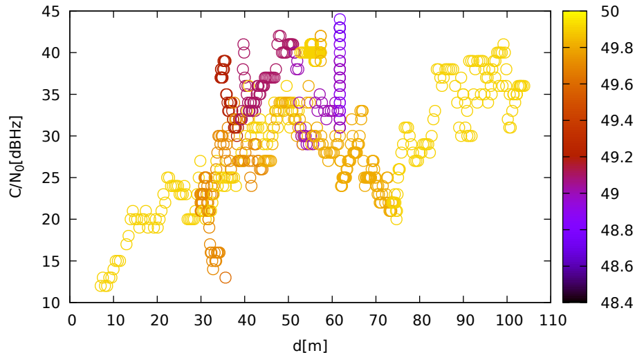
C/N 0 vs distance (ublox9 at C 1 for G14 at L1)
