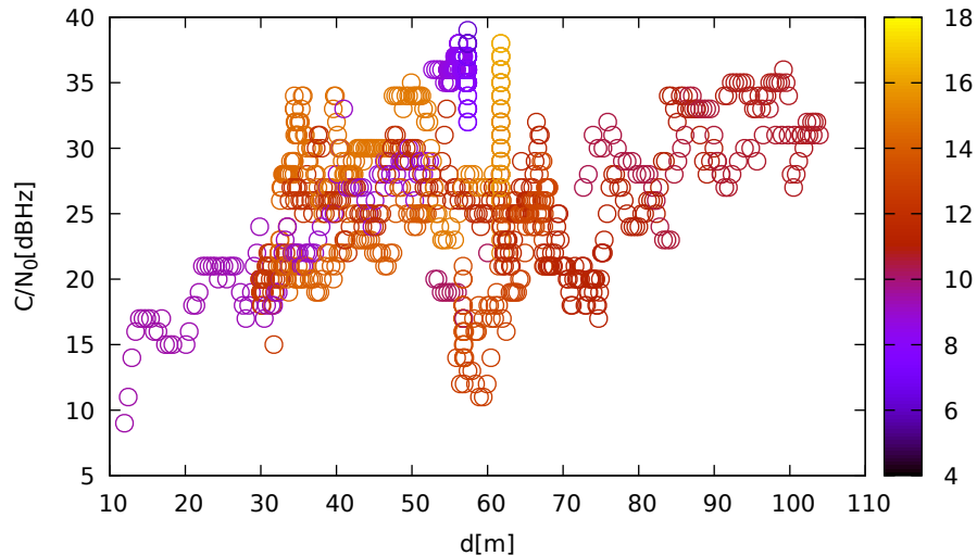
C/N_0 vs distance (ublox9 at C_1 for G17 at L1)
