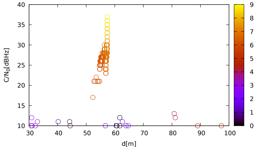
C/N 0 vs distance (ublox9 at C 1 for G21 at L1)
