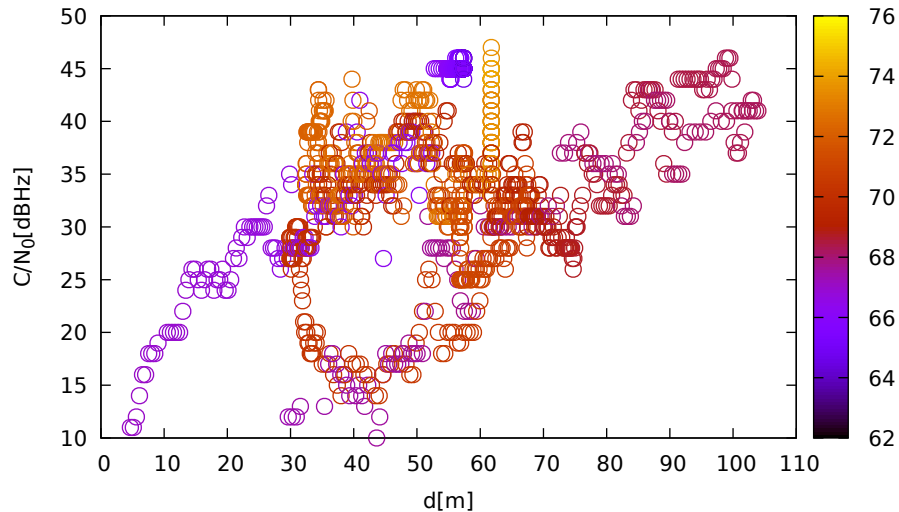
C/N 0 vs distance (ublox9 at C 1 for G22 at L1)
