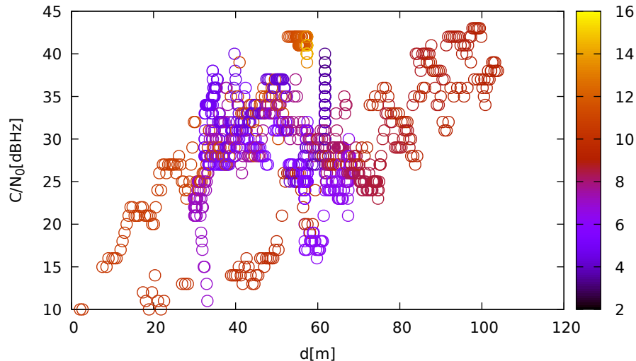
C/N 0 vs distance (ublox9 at C 1 for G27 at L1)
