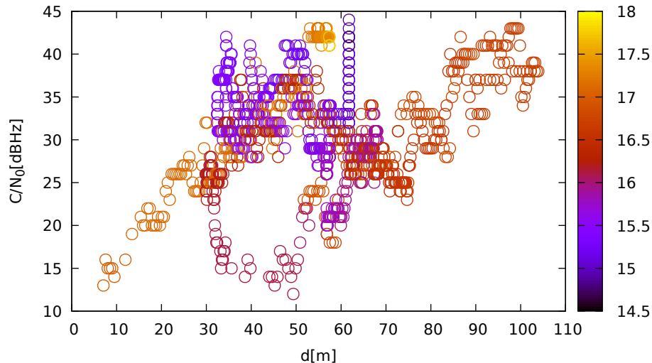
C/N 0 vs distance (ublox9 at C 1 for G28 at L1)
