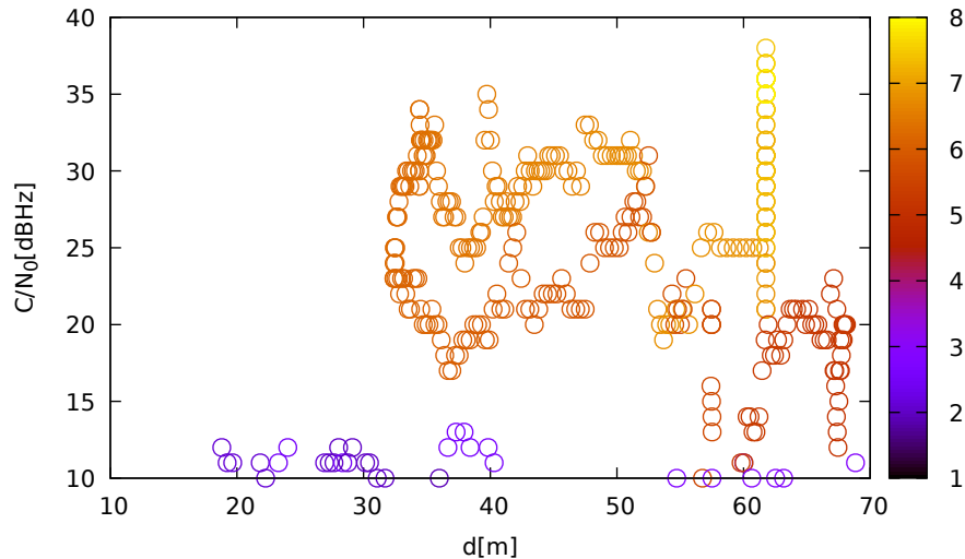
C/N 0 vs distance (ublox9 at C 1 for G31 at L1)
