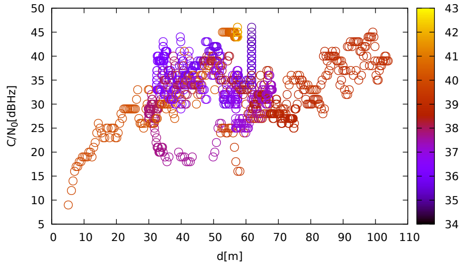
C/N 0 vs distance (ublox9 at C 1 for G32 at L1)
