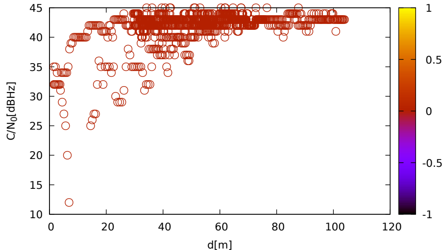
C/N_0 vs distance (ublox9 at C_1 for R06 at L1)
