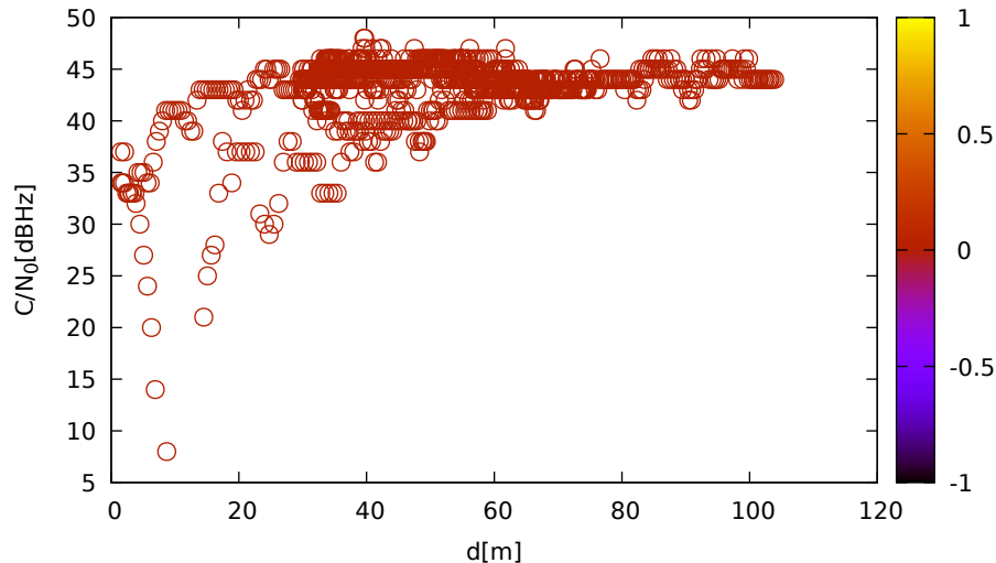
C/N_0 vs distance (ublox9 at C_1 for R07 at L1)
