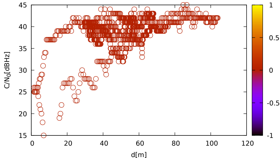
C/N 0 vs distance (ublox9 at C 1 for R14 at L1)
