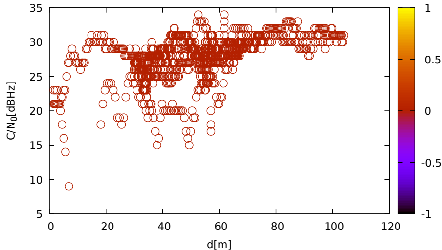
C/N 0 vs distance (ublox9 at C 1 for R15 at L1)
