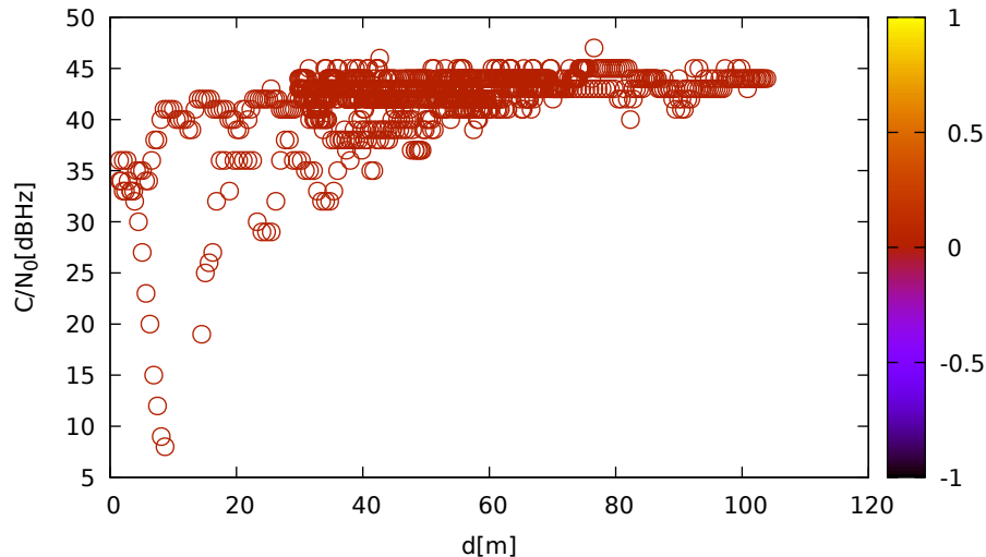
C/N_0 vs distance (ublox9 at C_1 for R21 at L1)
