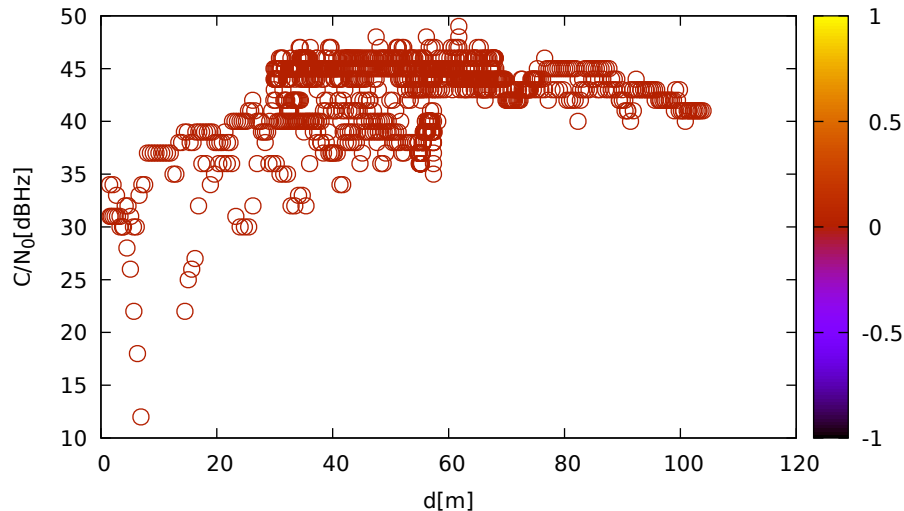
C/N_0 vs distance (ublox9 at C_1 for R23 at L1)
