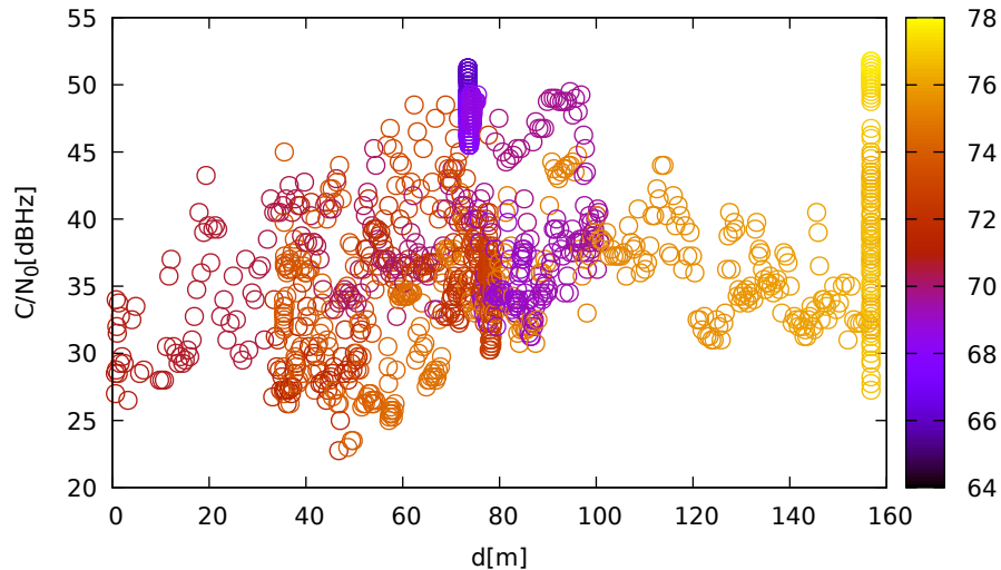
C/N 0 vs distance (JavadLSA at C 2 for G01 at L1)
