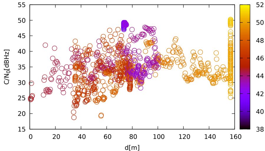
C/N 0 vs distance (JavadLSA at C 2 for G03 at L1)
