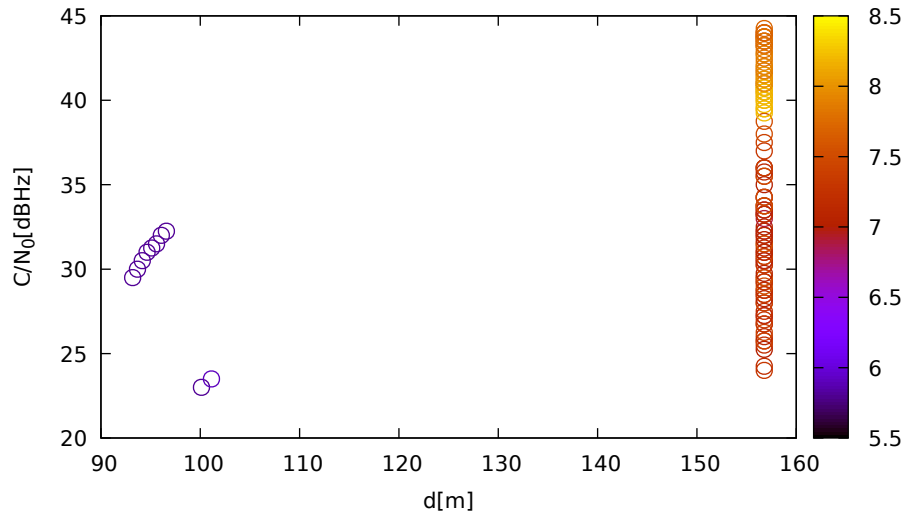
C/N 0 vs distance (JavadLSA at C 2 for G04 at L1)
