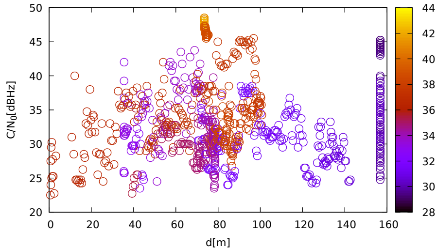
C/N 0 vs distance (JavadLSA at C 2 for G08 at L1)
