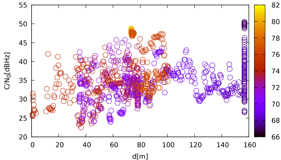
C/N 0 vs distance (JavadLSA at C 2 for G11 at L1)
