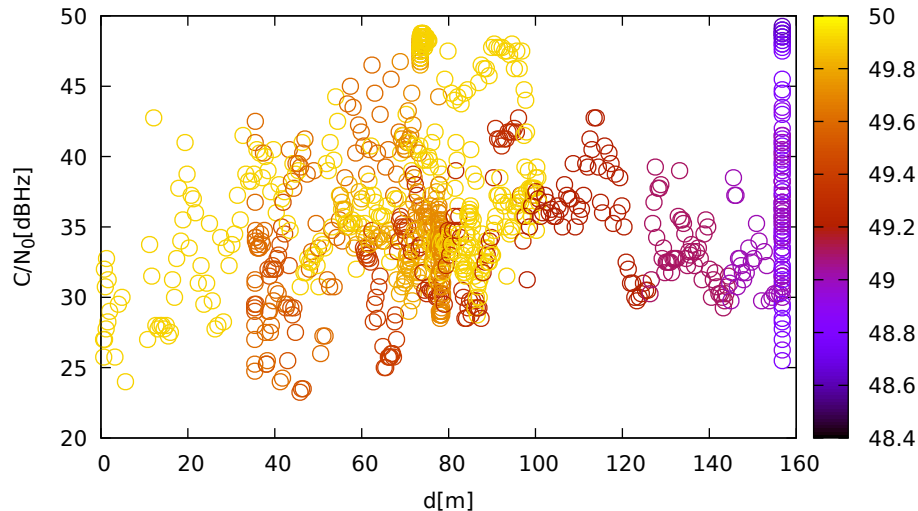
C/N 0 vs distance (JavadLSA at C 2 for G14 at L1)
