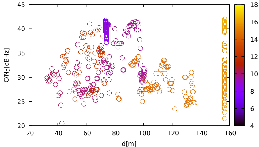
C/N 0 vs distance (JavadLSA at C 2 for G17 at L1)
