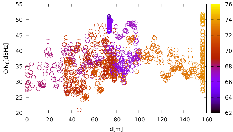
C/N 0 vs distance (JavadLSA at C 2 for G22 at L1)
