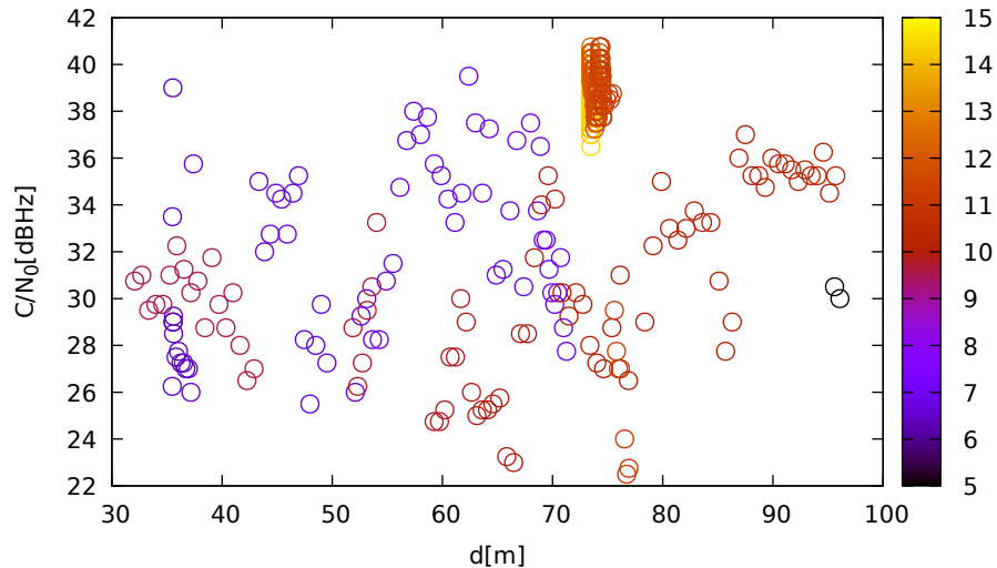
C/N 0 vs distance (JavadLSA at C 2 for G27 at L1)
