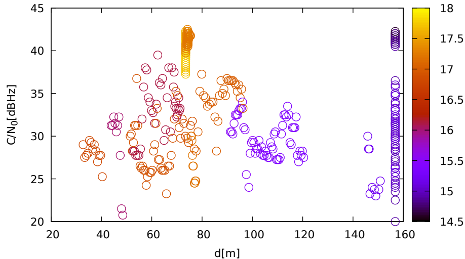
C/N 0 vs distance (JavadLSA at C 2 for G28 at L1)
