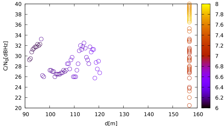
C/N 0 vs distance (JavadLSA at C 2 for G31 at L1)
