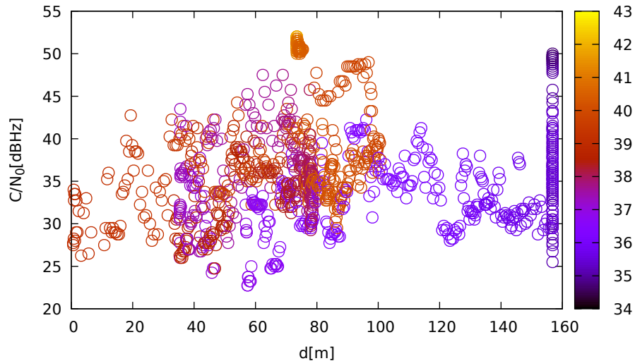
C/N 0 vs distance (JavadLSA at C 2 for G32 at L1)
