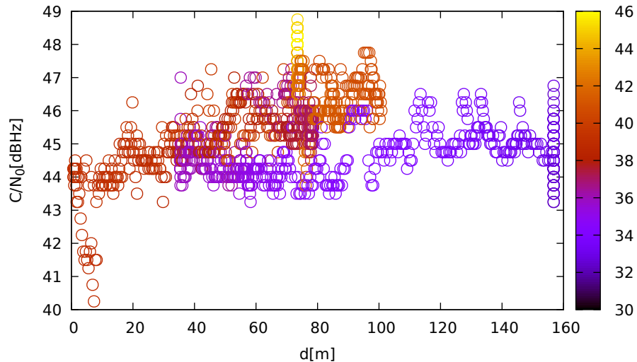
C/N 0 vs distance (JavadLSA at C 2 for R06 at L1)
