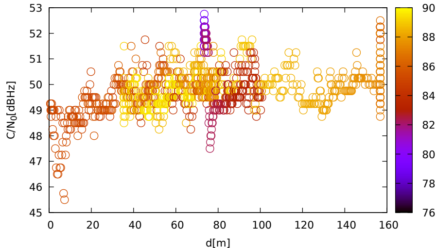
C/N 0 vs distance (JavadLSA at C 2 for R07 at L1)
