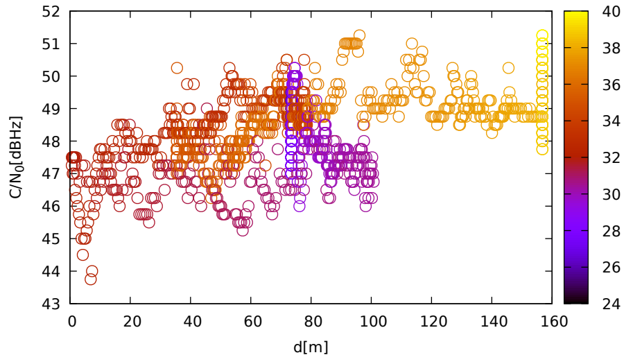
C/N 0 vs distance (JavadLSA at C 2 for R08 at L1)
