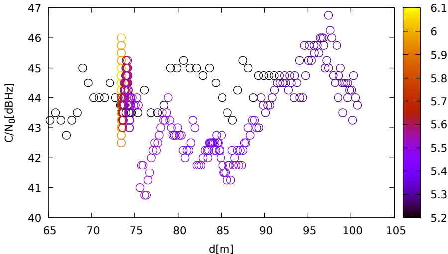
C/N 0 vs distance (JavadLSA at C 2 for R14 at L1)
