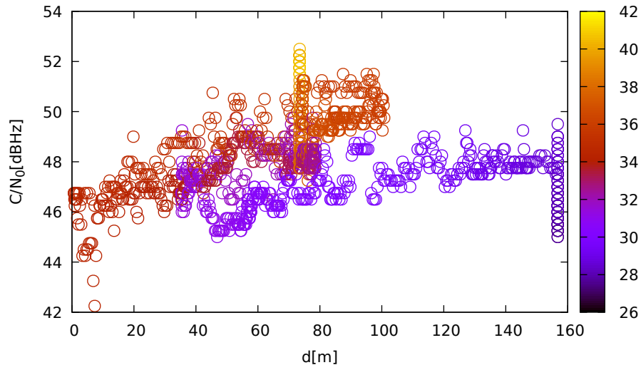
C/N 0 vs distance (JavadLSA at C 2 for R21 at L1)
