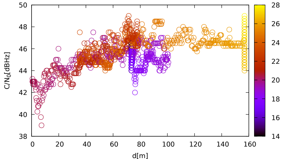
C/N 0 vs distance (JavadLSA at C 2 for R23 at L1)
