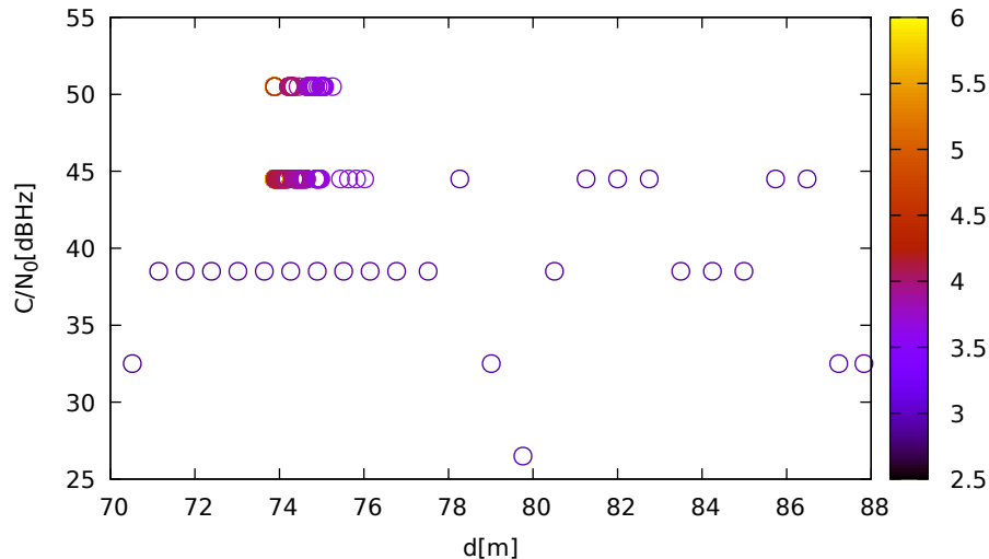
C/N 0 vs distance (LeicaGS15 at C 2 for E02 at L1)
