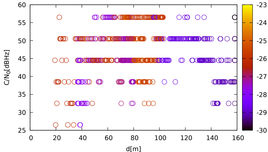
C/N 0 vs distance (LeicaGS15 at C 2 for E04 at L1)
