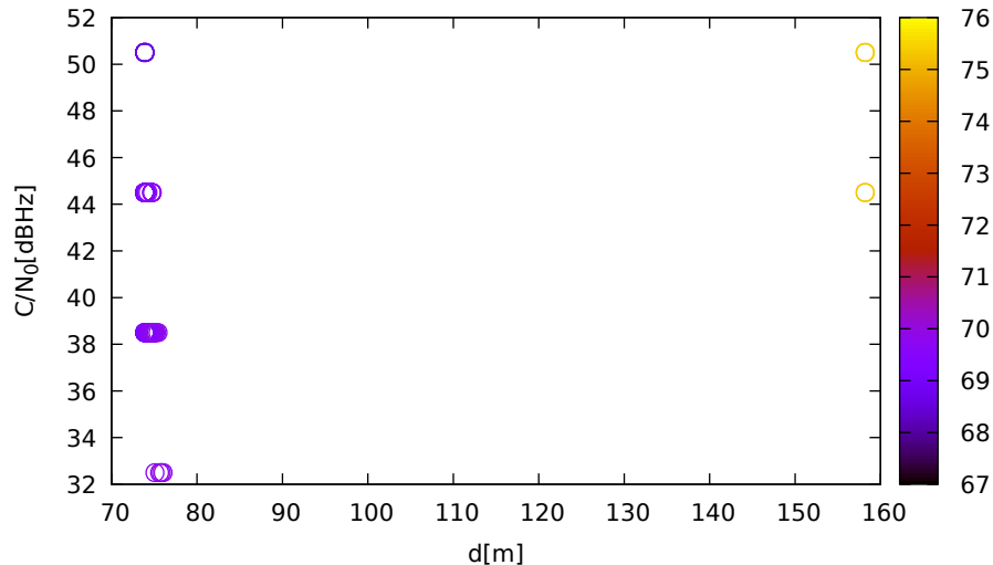
C/N 0 vs distance (LeicaGS15 at C 2 for E05 at L1)
