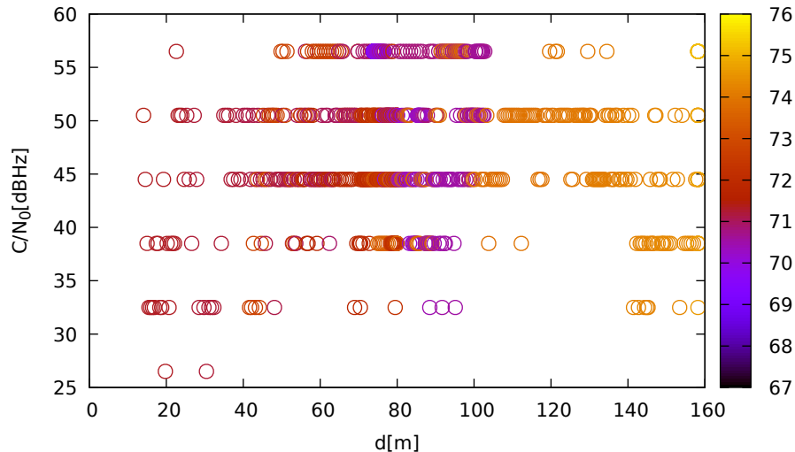
C/N 0 vs distance (LeicaGS15 at C 2 for E09 at L1)
