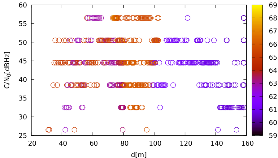
C/N 0 vs distance (LeicaGS15 at C 2 for E11 at L1)
