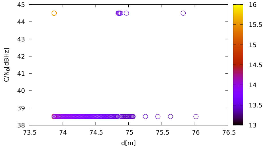
C/N 0 vs distance (LeicaGS15 at C 2 for E12 at L1)
