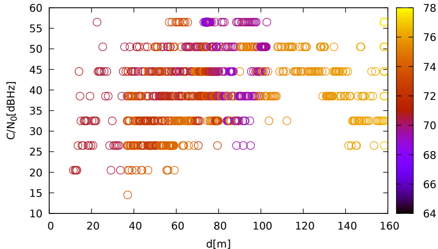
C/N 0 vs distance (LeicaGS15 at C 2 for G01 at L1)
