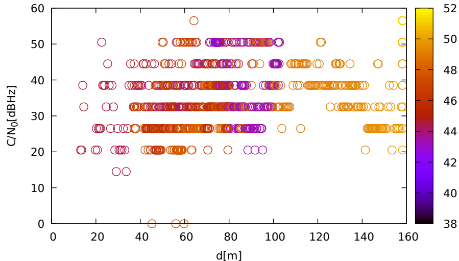
C/N 0 vs distance (LeicaGS15 at C 2 for G03 at L1)
