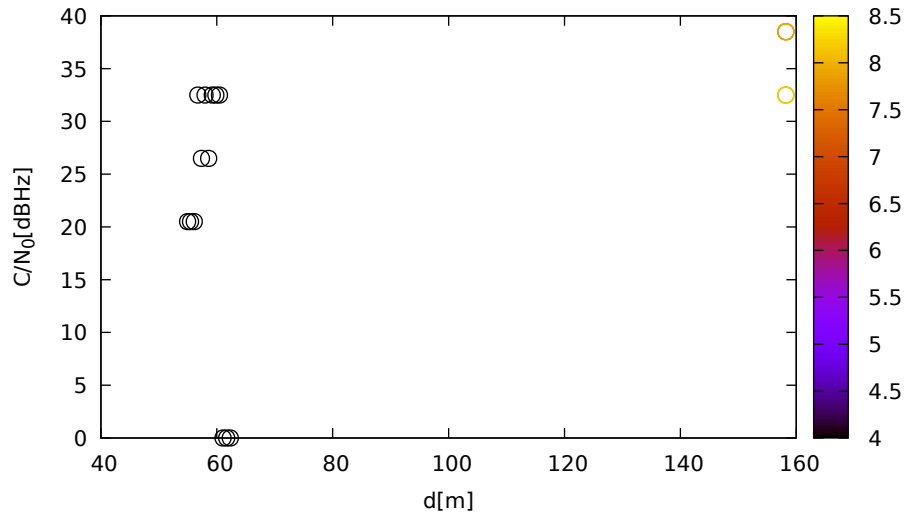
C/N 0 vs distance (LeicaGS15 at C 2 for G04 at L1)
