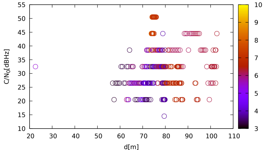
C/N 0 vs distance (LeicaGS15 at C 2 for G10 at L1)
