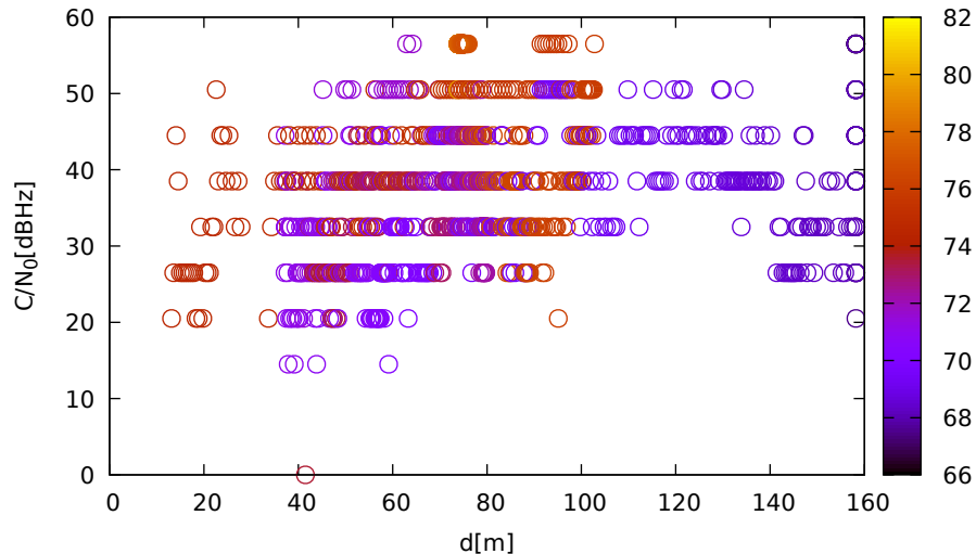
C/N 0 vs distance (LeicaGS15 at C 2 for G11 at L1)
