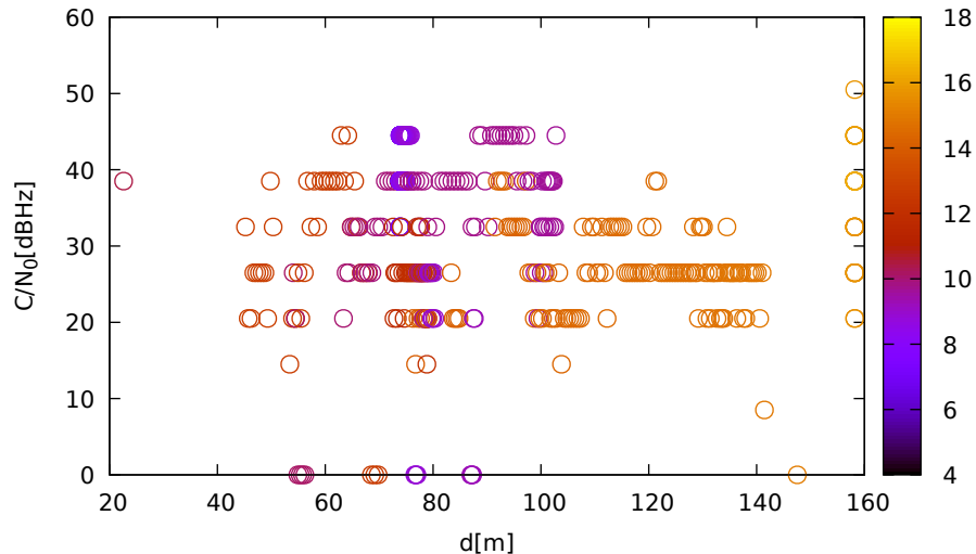
C/N 0 vs distance (LeicaGS15 at C 2 for G17 at L1)
