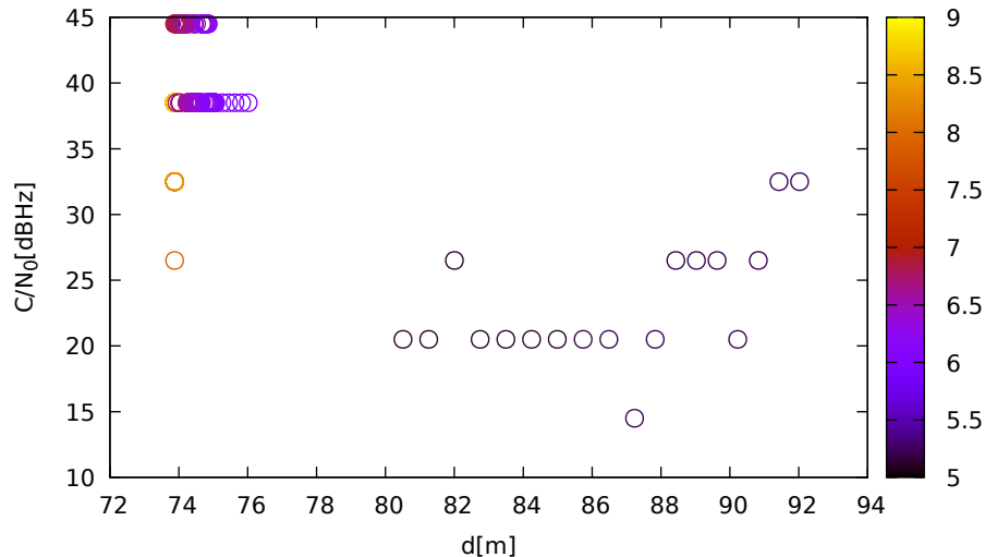
C/N 0 vs distance (LeicaGS15 at C 2 for G21 at L1)
