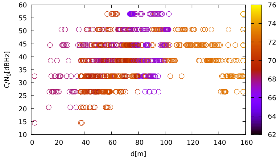
C/N 0 vs distance (LeicaGS15 at C 2 for G22 at L1)
