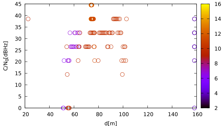
C/N 0 vs distance (LeicaGS15 at C 2 for G27 at L1)
