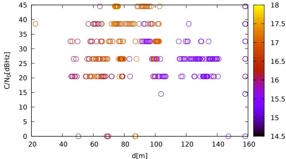
C/N 0 vs distance (LeicaGS15 at C 2 for G28 at L1)
