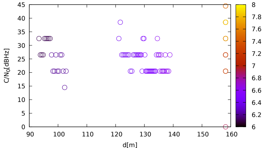
C/N 0 vs distance (LeicaGS15 at C 2 for G31 at L1)
