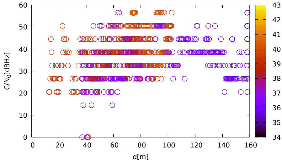
C/N 0 vs distance (LeicaGS15 at C 2 for G32 at L1)
